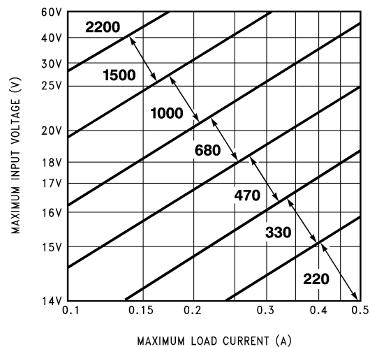
FIGURE 6. LM2574HV-12 Inductor Selection Guide
