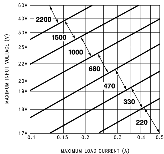
FIGURE 7. LM2574HV-15 Inductor Selection Guide
