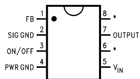
8-Lead DIP
