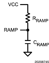
FIGURE 7. R_{RAMP} to V_{CC} for V_{OUT} > 7.5V
