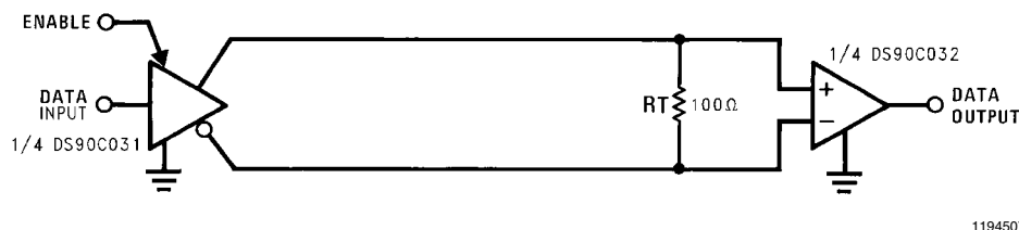
FIGURE 5. Point-to-Point Application
