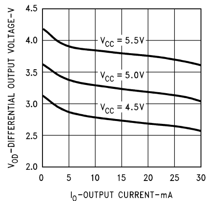
Driver V_{OD} vs V_{CC}
