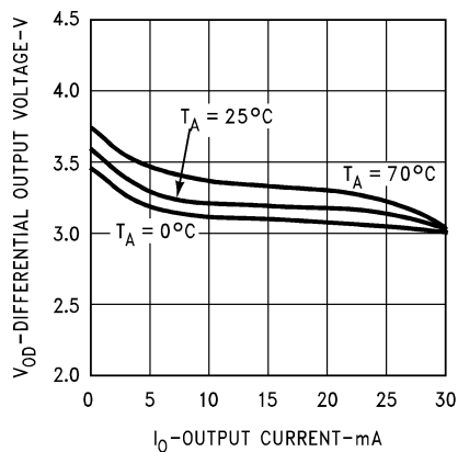
Driver V_{OD} vs Temperature
