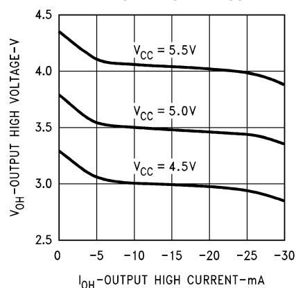
Driver V_{OH} vs I_{OH} vs V_{CC}
