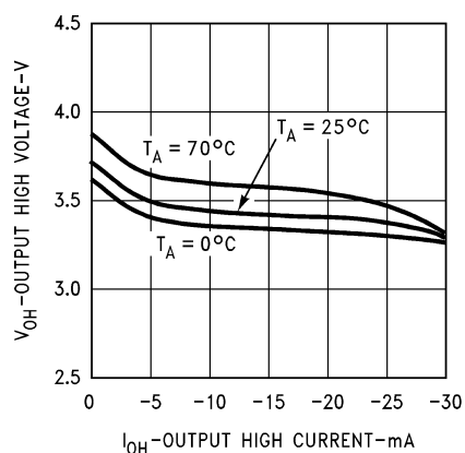
Driver V_{OH} vs I_{OH} vs Temperature
