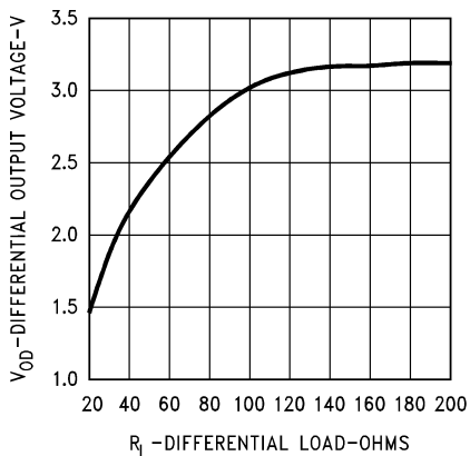
Driver V_{OD} vs R_L
