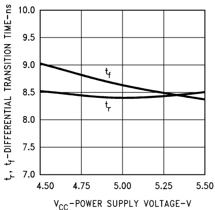
Driver Differential Transition Time vs V_{CC}
