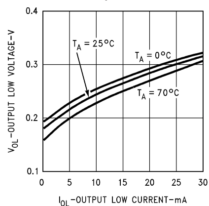
Driver V_{OL} vs I_{OL} vs Temperature
