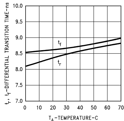
Driver Differential Transition Time vs Temperature
