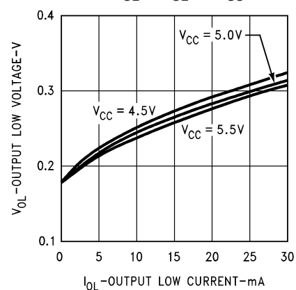
Driver V_{OL} vs I_{OL} vs V_{CC}
