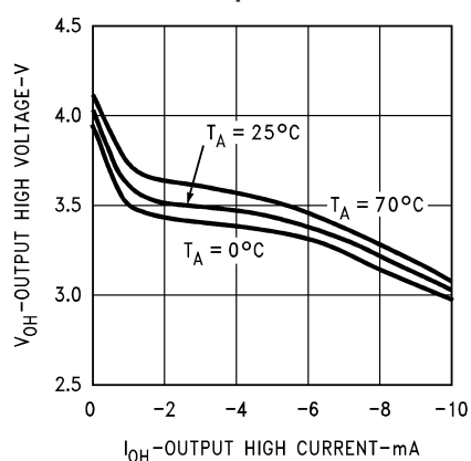
Receiver V_{OH} vs I_{OH} vs Temperature
