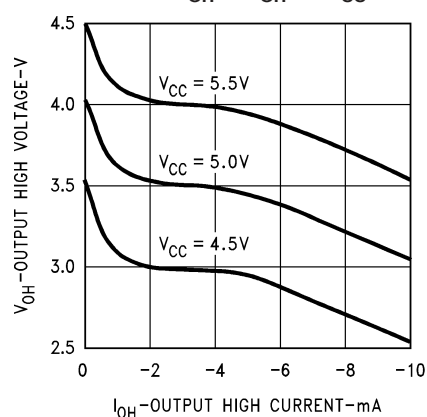
Receiver V_{OH} vs I_{OH} vs V_{CC}
