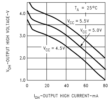
Output High Voltage vs Output High Current
