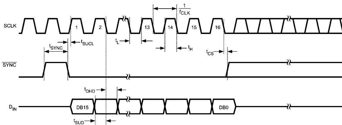
FIGURE 2. DAC081S101 Timing
