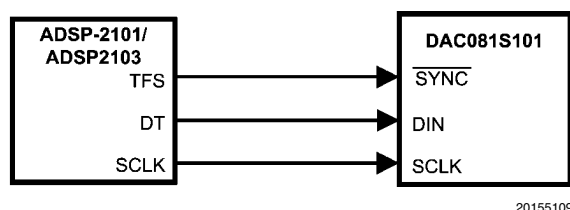
FIGURE 5. ADSP-2101/2103 Interface
