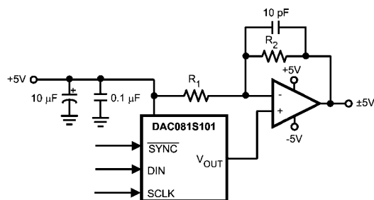
FIGURE 13. Bipolar Operation
