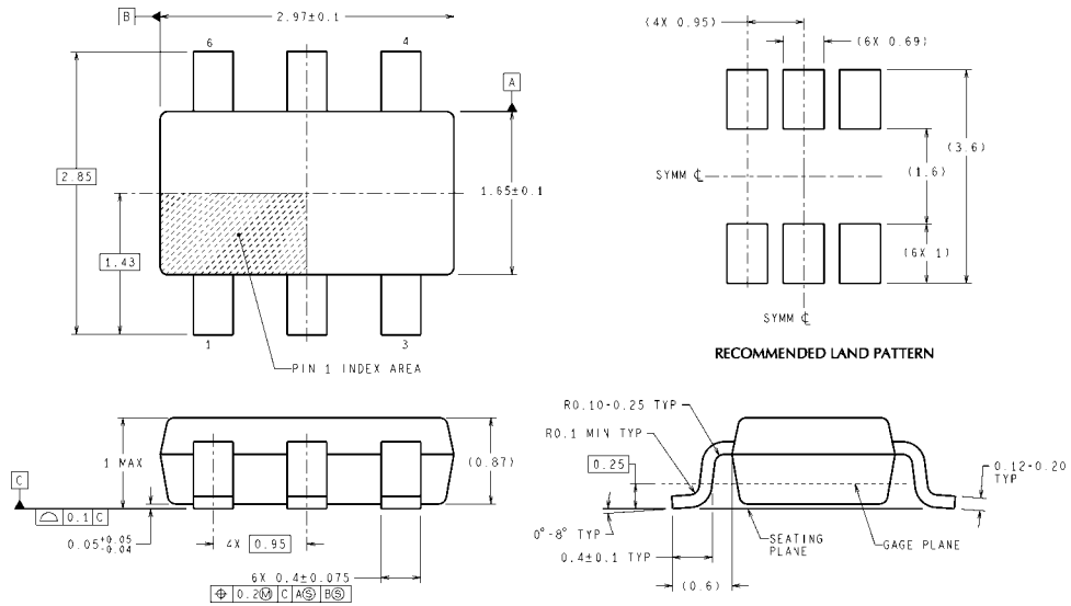
6-Lead TSOT Order Numbers DAC081S101CIMK NS Package Number MK06A
