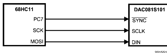
FIGURE 7. 68HC11 Interface
