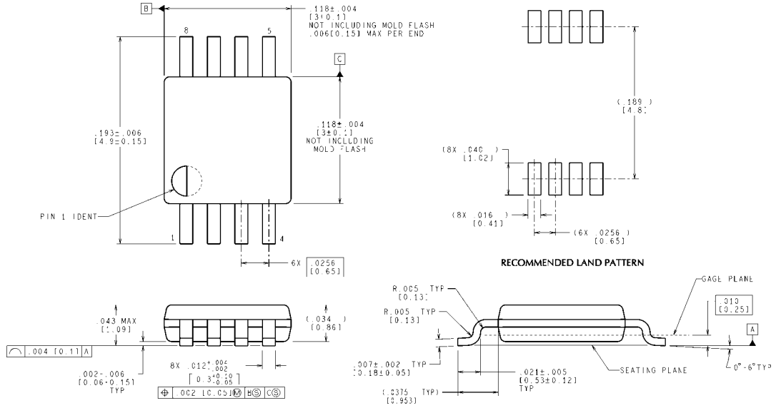
8-Lead MSOP Order Numbers DAC081S101CIMM NS Package Number MUA08A
