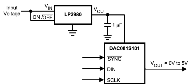
FIGURE 12. Using the LP2980 regulator
