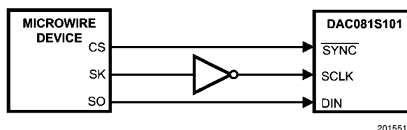
FIGURE 8. Microwire Interface
