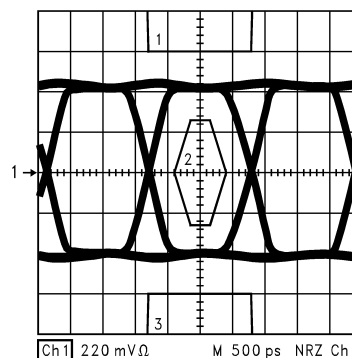
10132910 622 Mbps Eye Pattern with STM-4 Signal Mask
