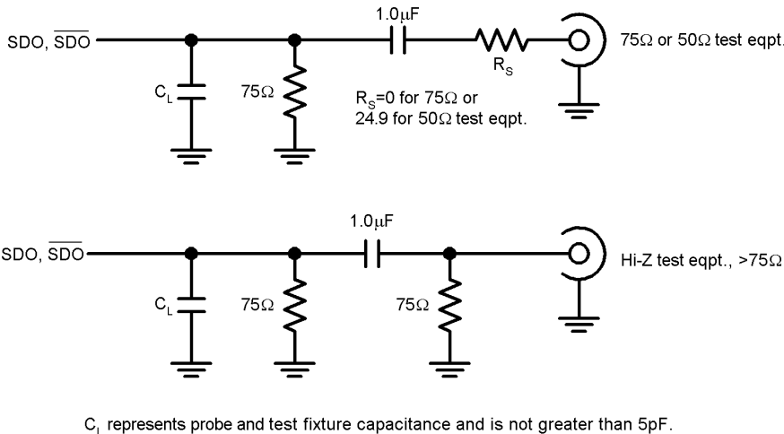
FIGURE 1. Test Loads
