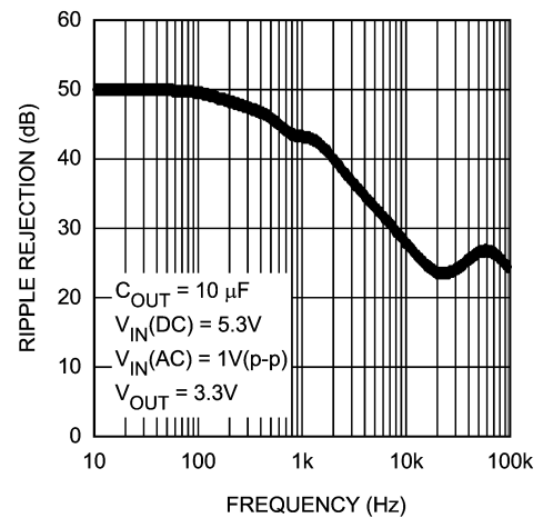
Ripple Rejection
