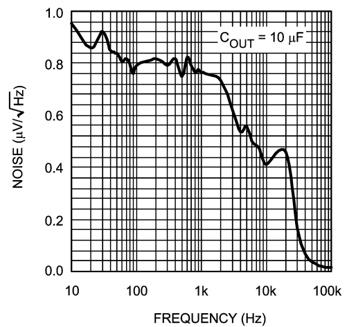
Noise vs Frequency
