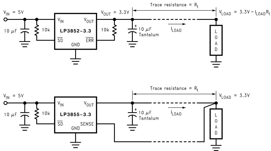
FIGURE 2. Improving remote load regulation using LP3855
