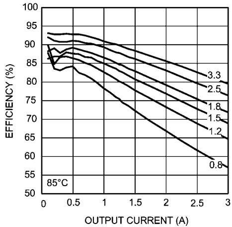
Efficiency 6V Input @ 85°C
