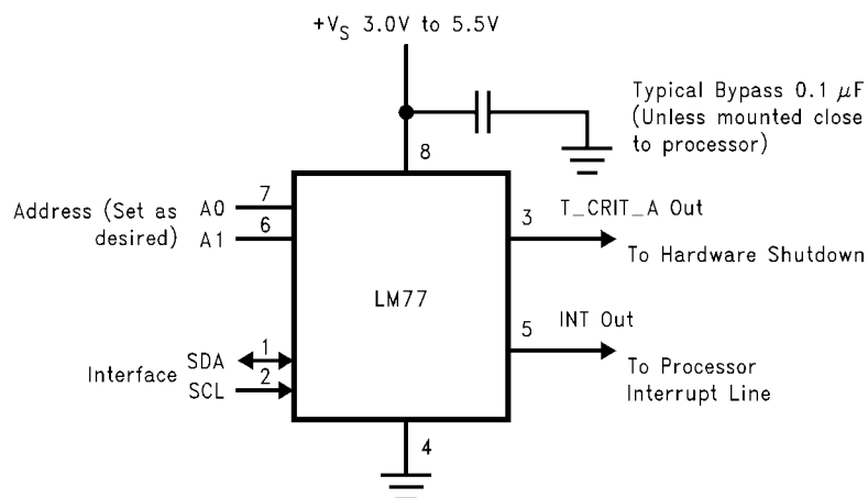
FIGURE 1. Typical Application
