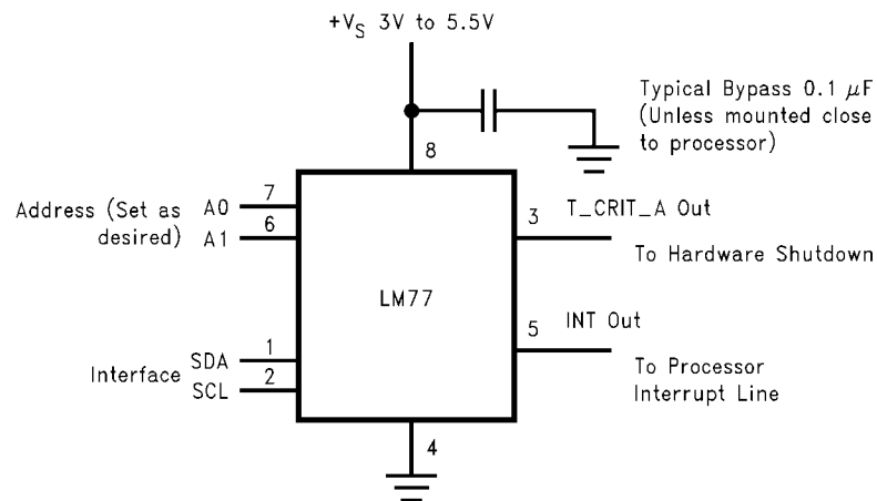
FIGURE 8. Typical Application
