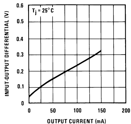
Dropout Voltage
