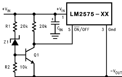
FIGURE 12. Undervoltage Lockout for Buck Circuit
