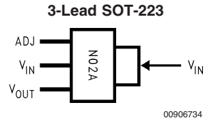
Front View Order Number LM337IMP Package Marked N02A See NS Package Number MP04A
