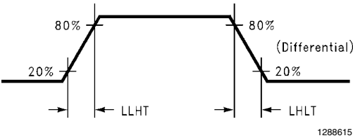
FIGURE 3. DS90C363 (Transmitter) LVDS Output Load and Transition Times
