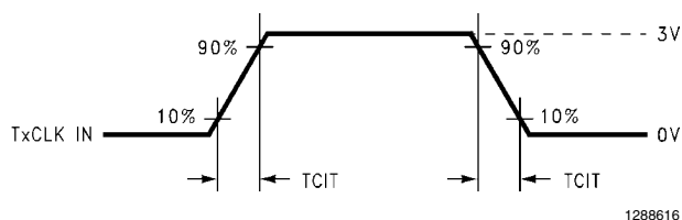
FIGURE 5. DS90C363 (Transmitter) Input Clock Transition Time
