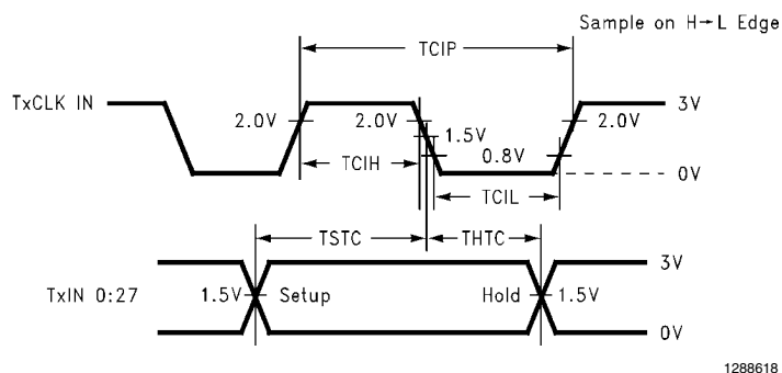
FIGURE 7. DS90C363 (Transmitter) Setup/Hold and High/Low Times
