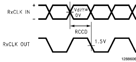
FIGURE 10. DS90CF364 (Receiver) Clock In to Clock Out Delay
