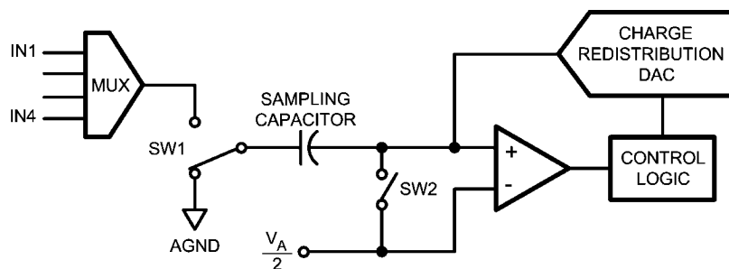
FIGURE 2. ADC124S021 in Hold Mode
