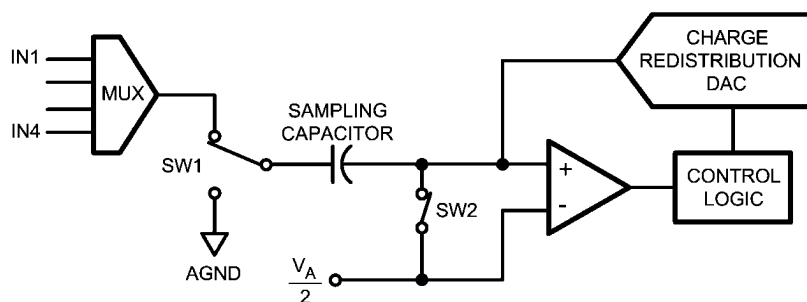
FIGURE 1. ADC124S021 in Track Mode
