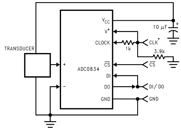
FIGURE 6. Generating V CC from the Converter Clock
