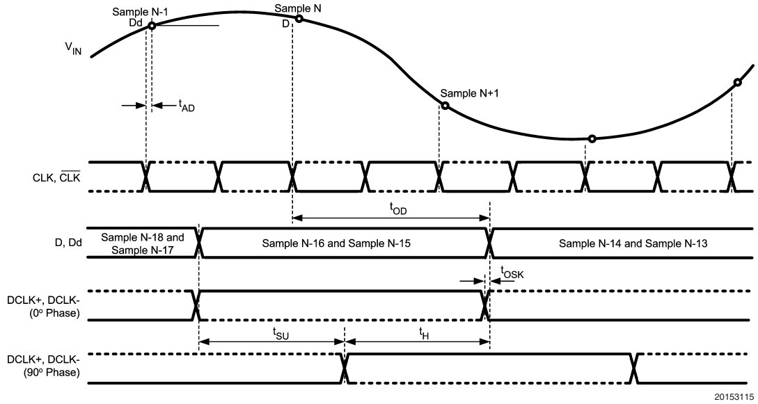
FIGURE 4. ADC081500 Timing — DDR Clcking
