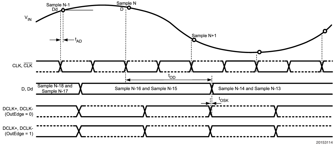
FIGURE 3. ADC081500 Timing — SDR Clcking
