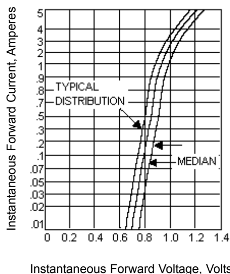
Figure 3 - Typical Forward Characteristics (25°C)
