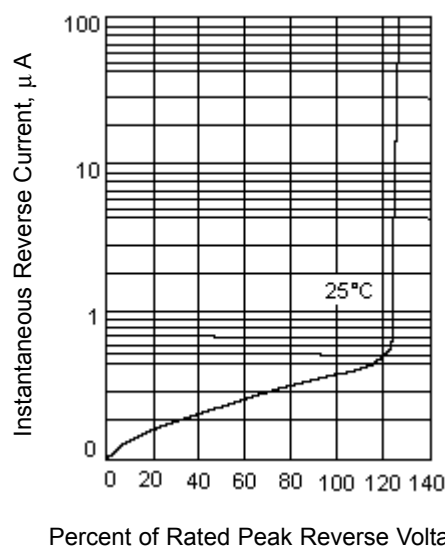
Figure 4 - Reverse Characteristics
