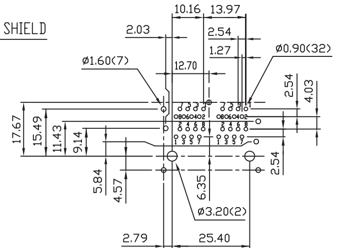
PCB LAYOUT
