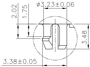
DETAIL X
