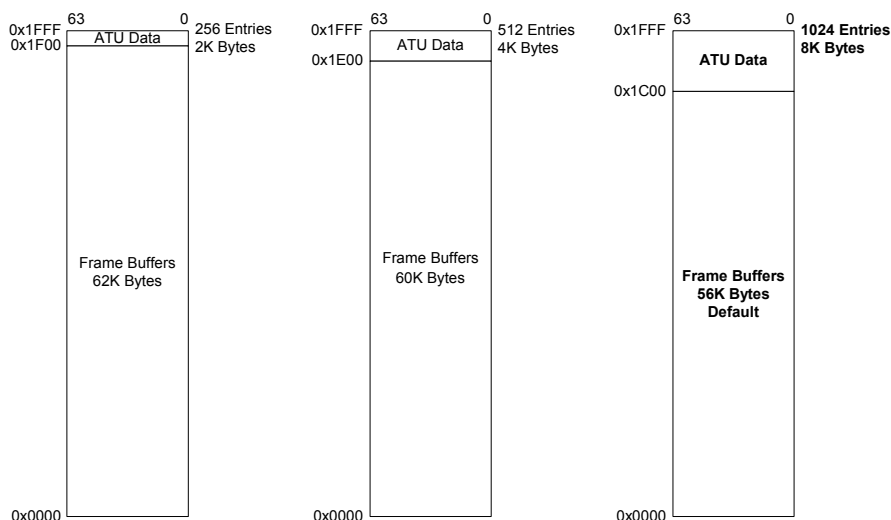
Figure 11: ATU Size Tradeoffs
