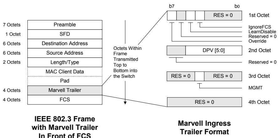
Figure 15: Ingress Trailer Format
