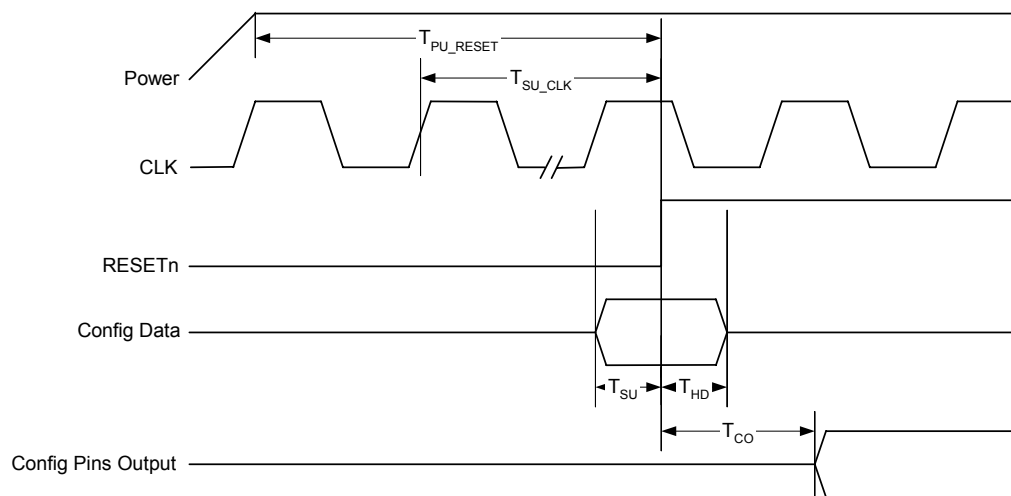
Figure 28: Reset and Configuration Timing
