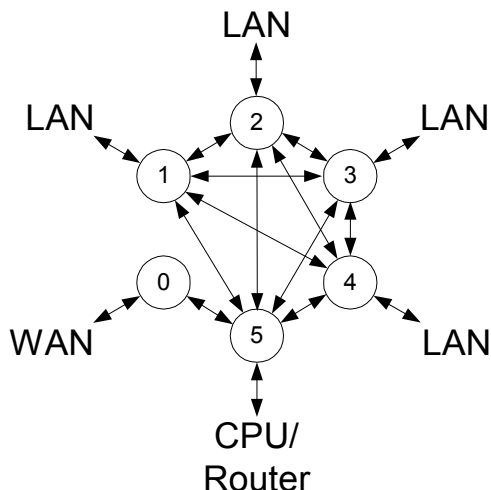
Figure 14: Switch Operation with a Typical Router VLAN Configuration
