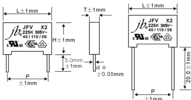
Dimensions Table for 305V AC:
