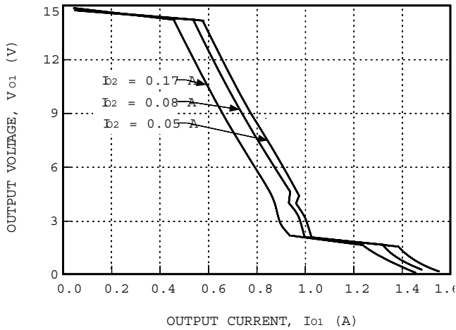
Figure 9. MH005CL Typical Output Characteristics with V_I = 12\text{ V} and T_A = 25\text{ }^\circ\text{C}
