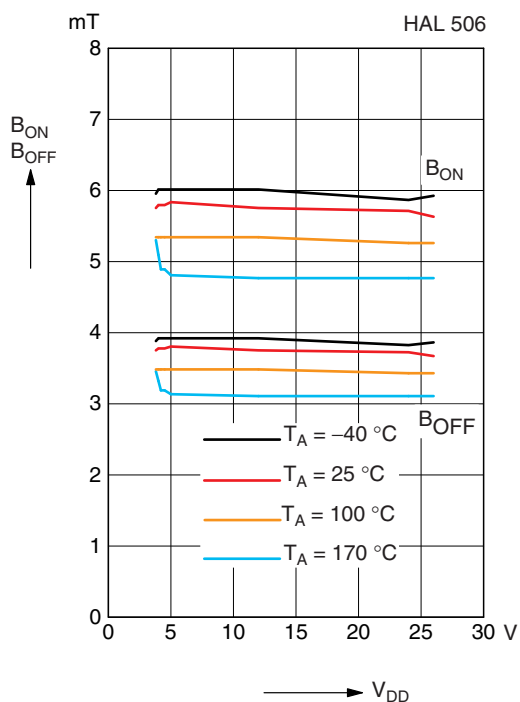
Fig. 4-22: Typ. magnetic switching points versus supply voltage
