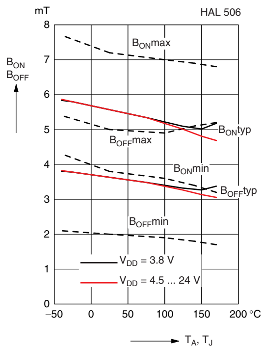
Fig. 4-24: Magnetic switching points versus temperature
