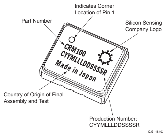
Figure 11.1 Part Marking
