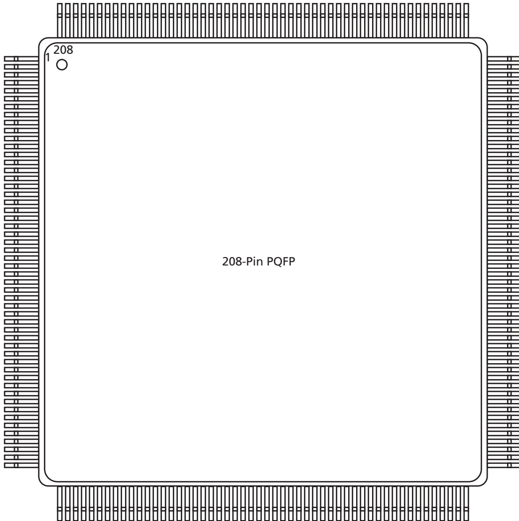
Figure A-1 • 208-Pin PQFP
