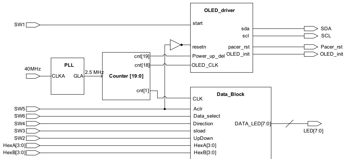
Figure 4-1 • Design Block Diagram
