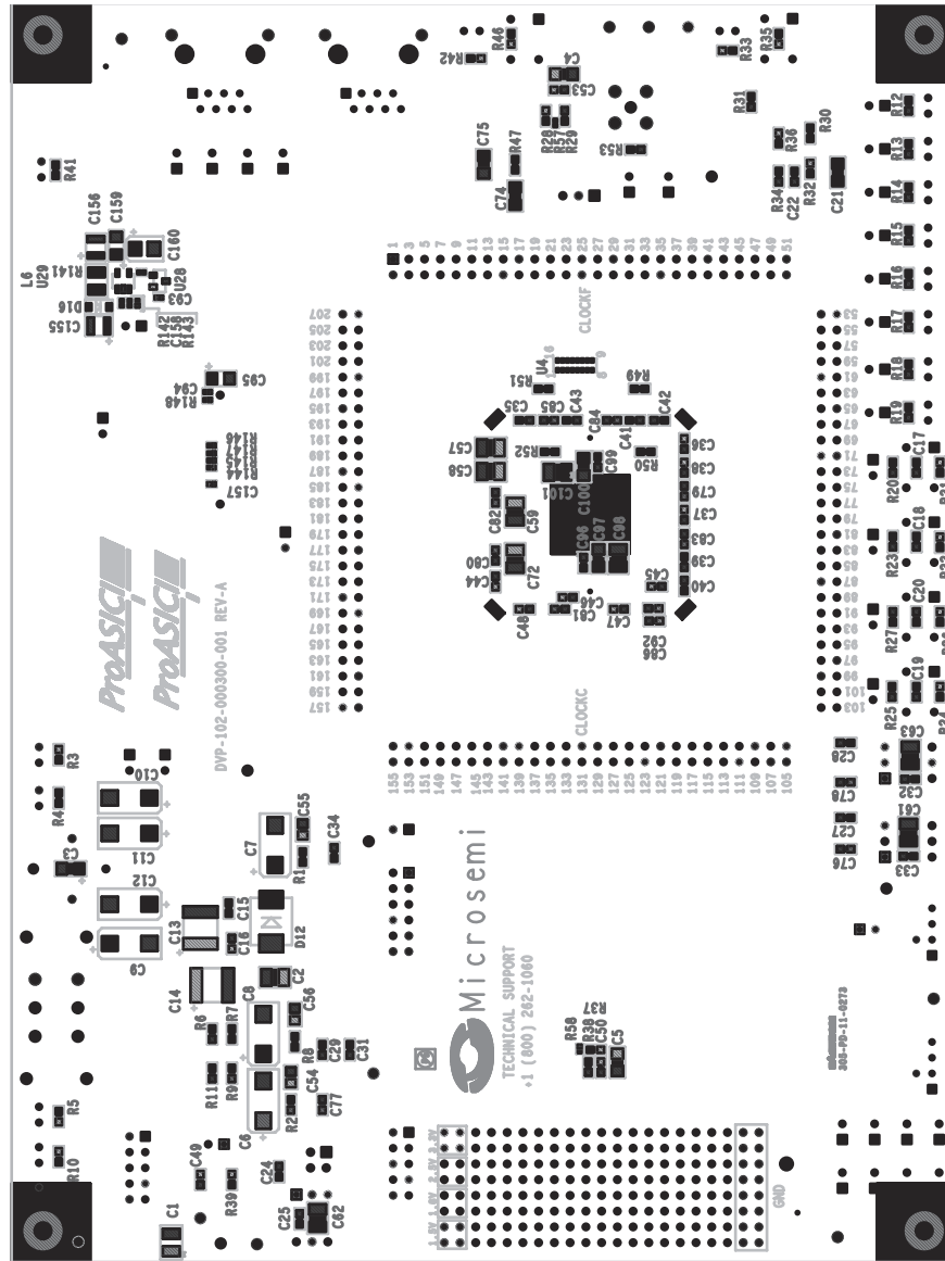
Figure B-2 • Bottom-Level View of ProASIC3/E Starter Kit Board
