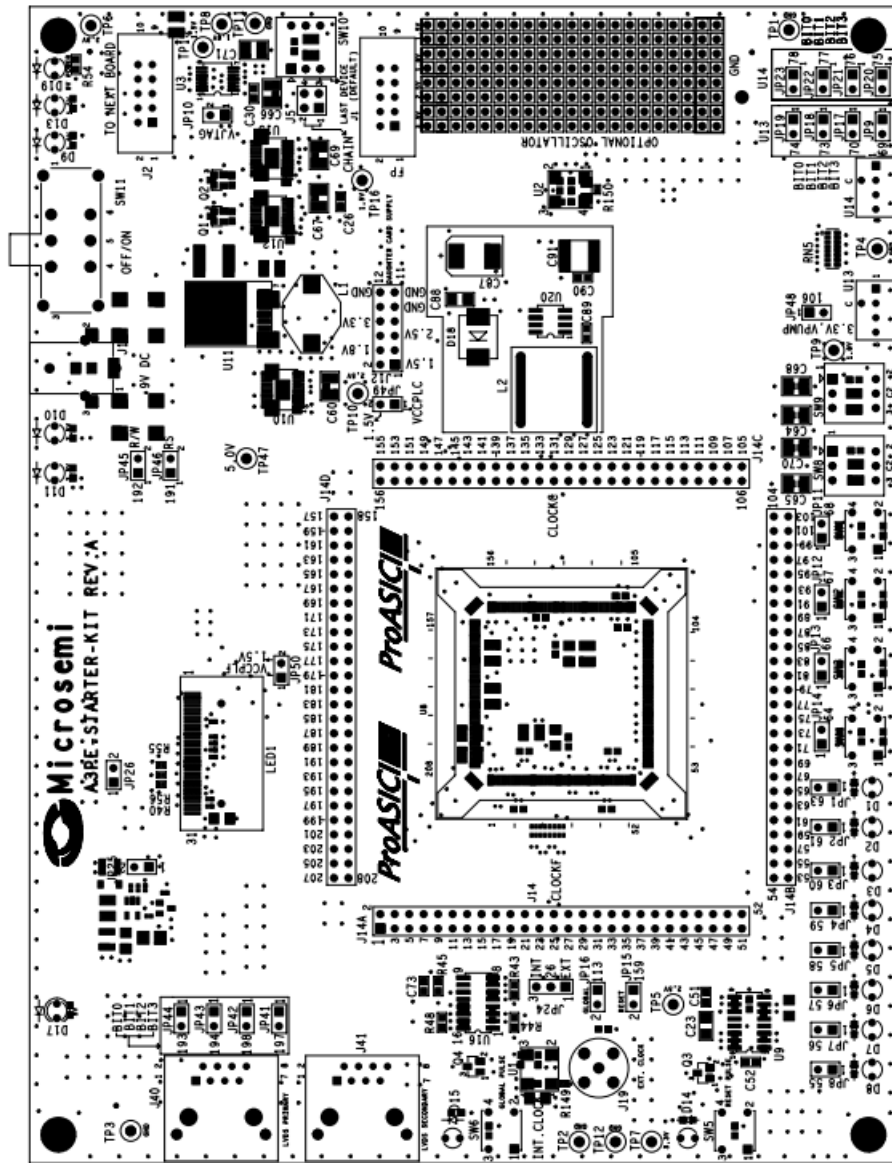
Figure 2-1 • ProASIC3/E Starter Kit Board: Top-Level View
