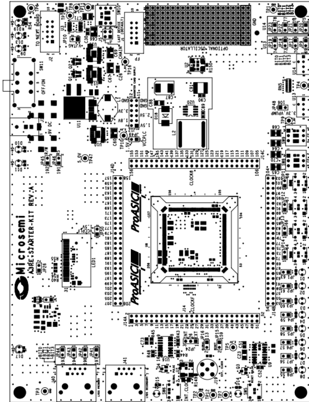
Figure B-1 • Top-Level View of ProASIC3/E Starter Kit Board
