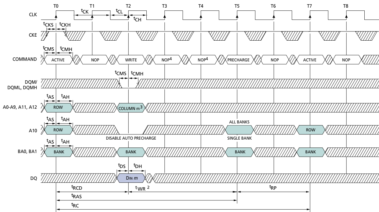
Figure 45: Single Write – Without Auto Precharge 1
