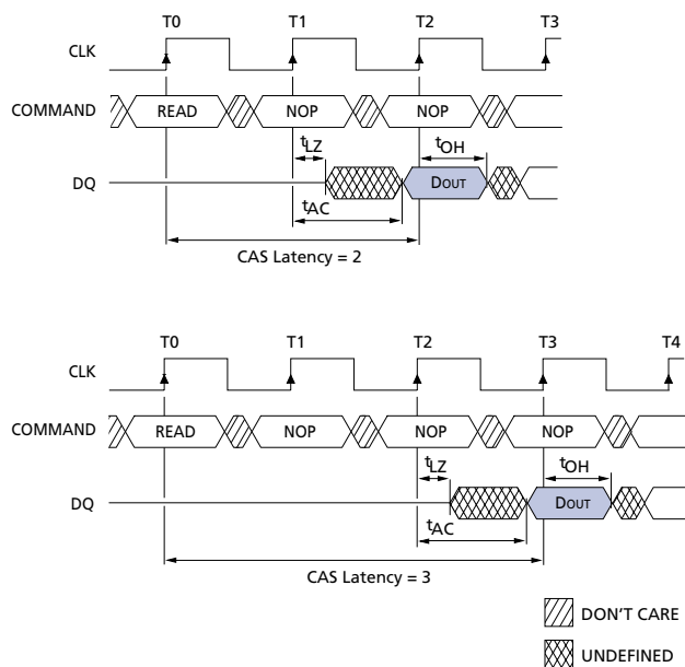
Figure 6: CAS Latency
