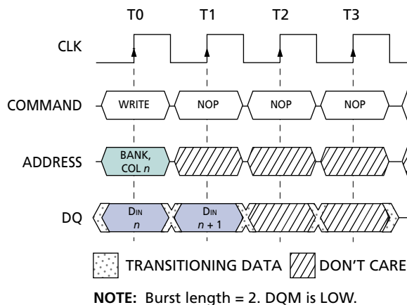
Figure 17: WRITE Burst
