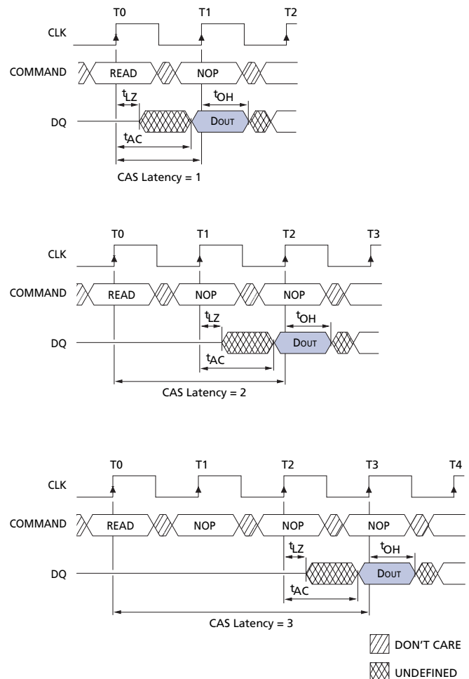
Figure 9: CAS Latency
