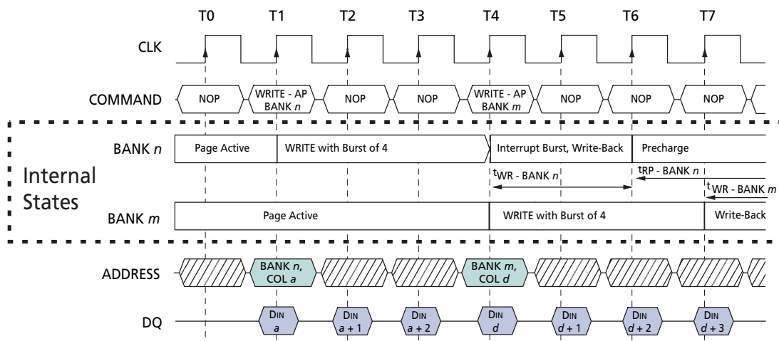
Figure 30: WRITE With Auto Precharge Interrupted by a WRITE
