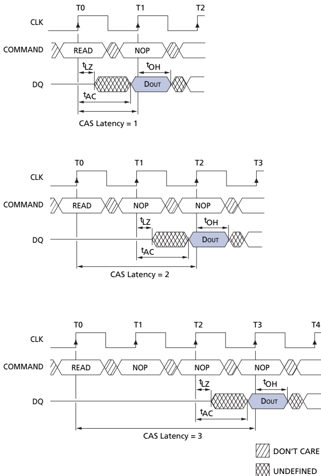
Figure 5: CAS Latency
