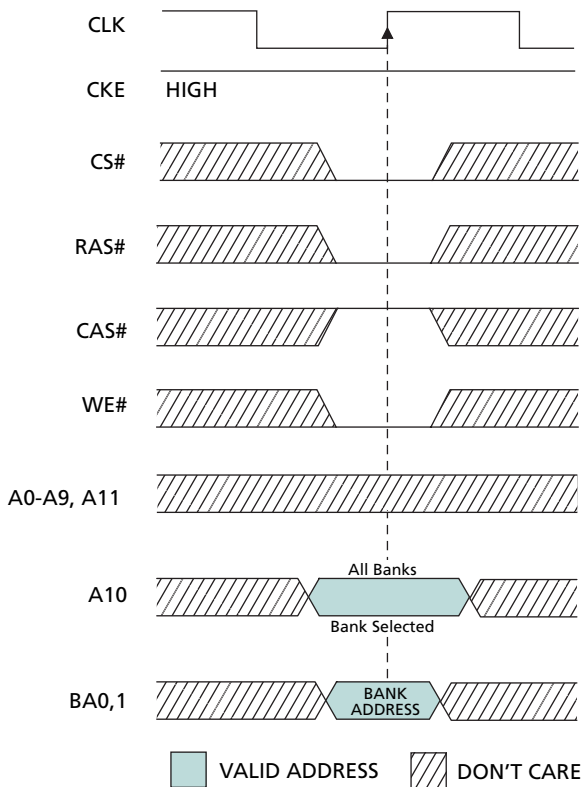
Figure 23: PRECHARGE Command
