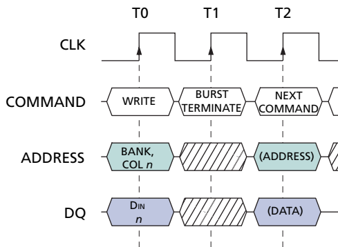
Figure 22: Terminating a WRITE Burst
