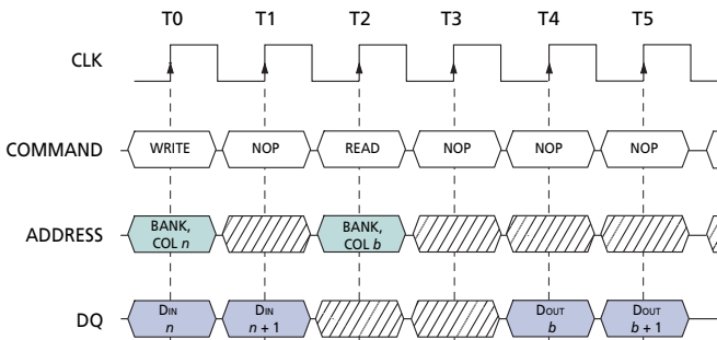
Figure 20: WRITE to READ
