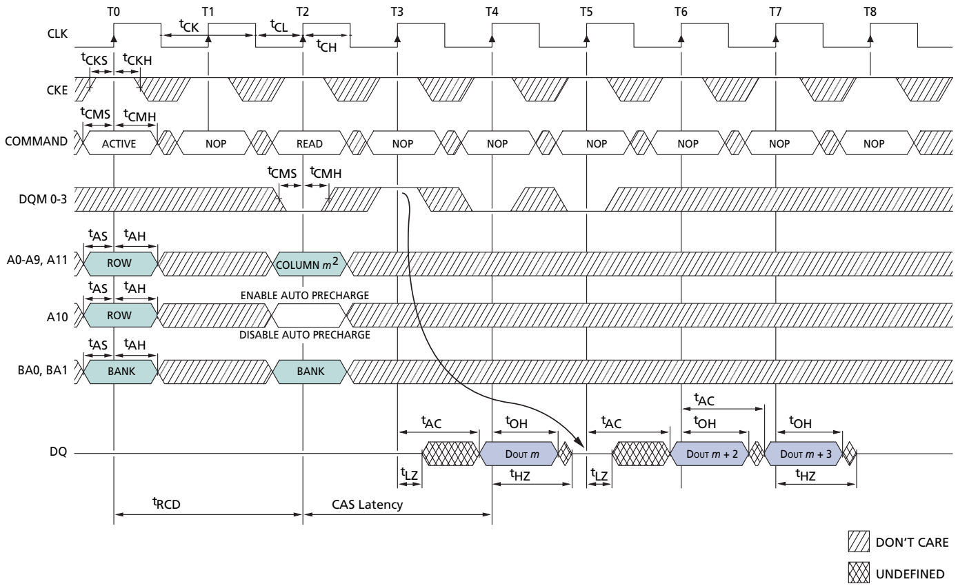
Figure 40: Read – DQM Operation
