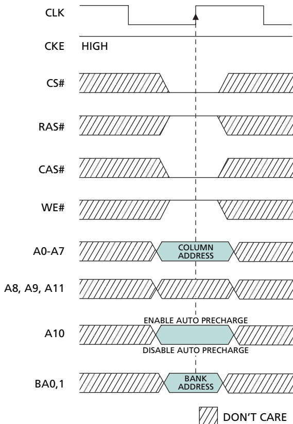
Figure 8: READ Command
