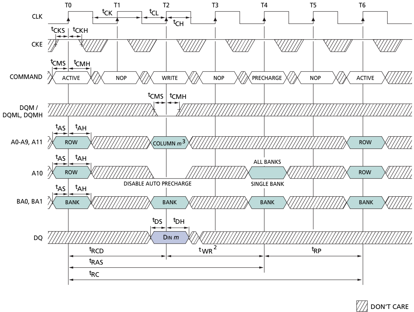
Figure 41: Single Write
