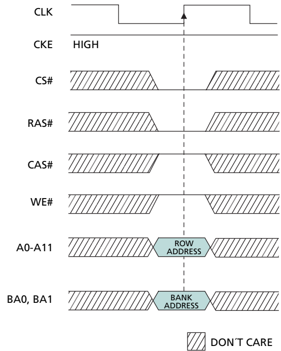
Figure 7: Example: Meeting t_{RCD}(\text{MIN}) When 2 < t_{RCD}(\text{MIN})/t_{CK} \leq 3
