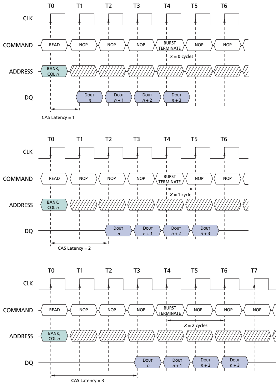
Figure 15: Terminating a READ Burst
