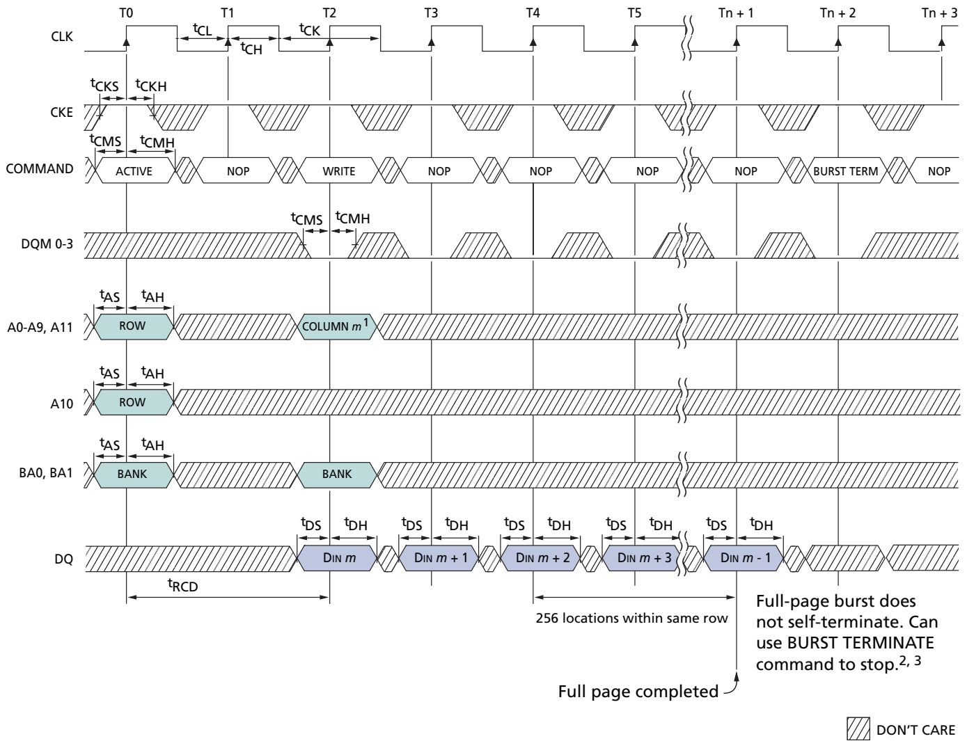
Figure 45: Write – Full-page Burst
