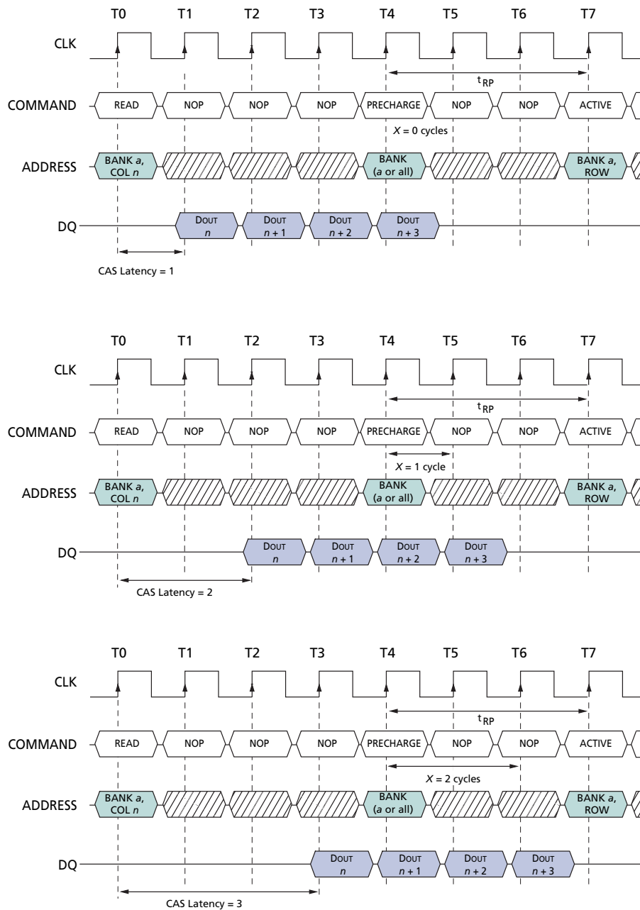
Figure 14: READ to PRECHARGE
