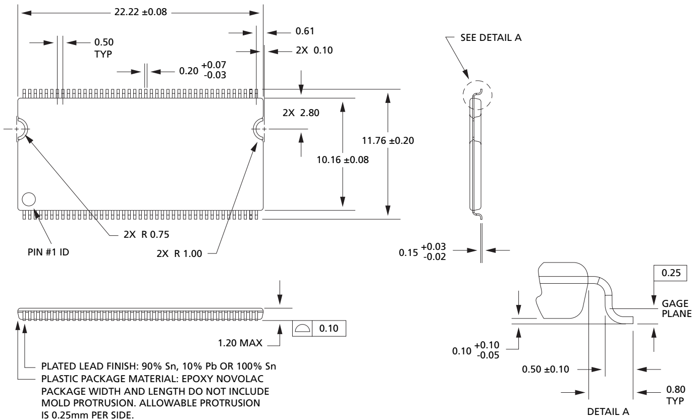
Figure 47: 86-Pin Plastic TSOP (400 mil)
