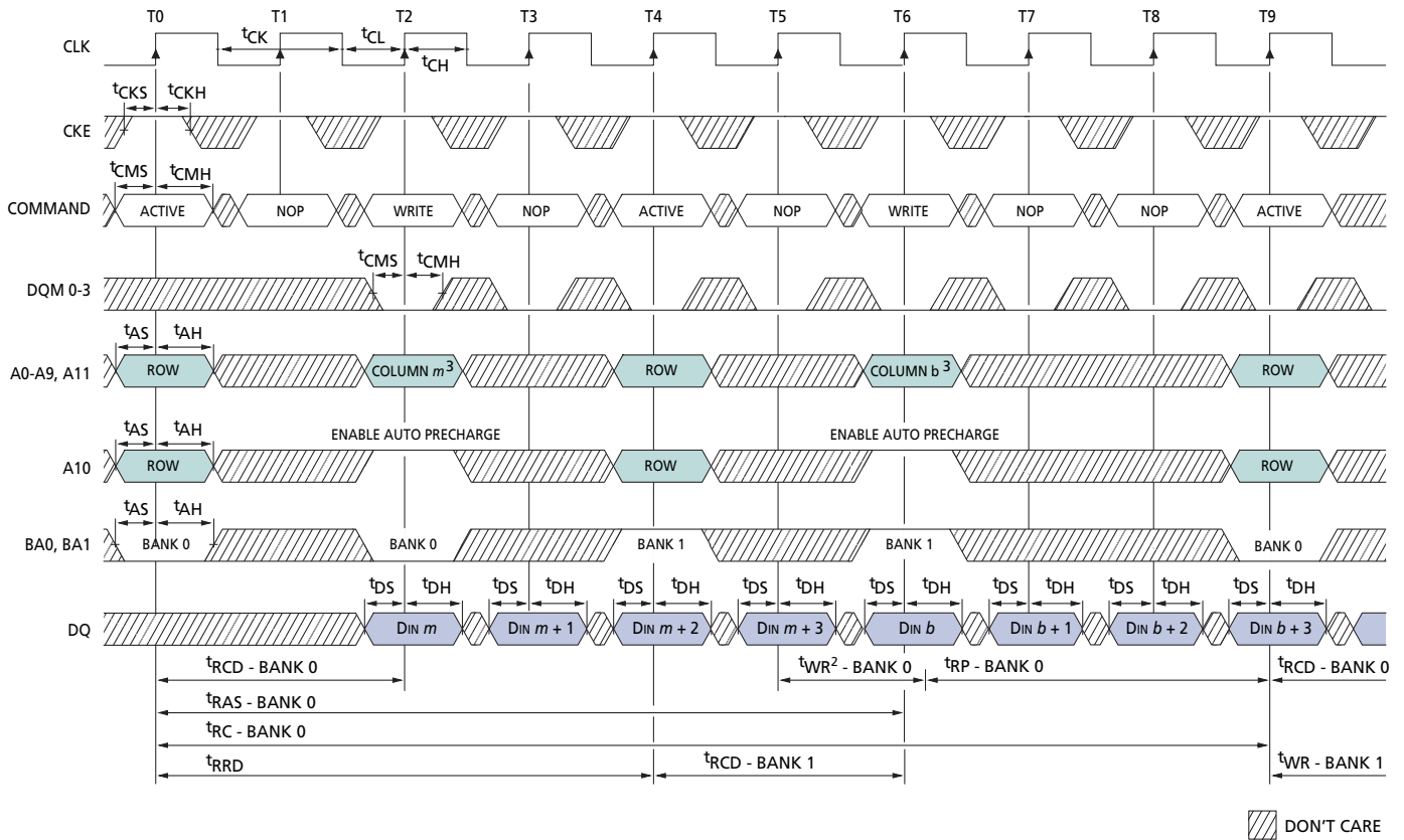
Figure 44: Alternating Bank Write Accesses
