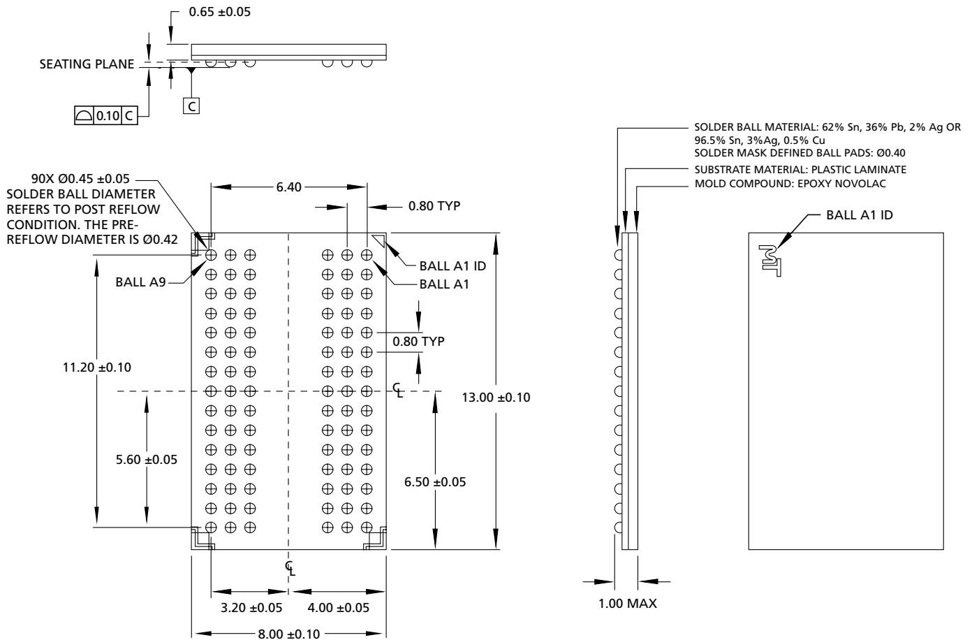
Figure 48: 90-Ball FBGA (8mm x 13mm)
