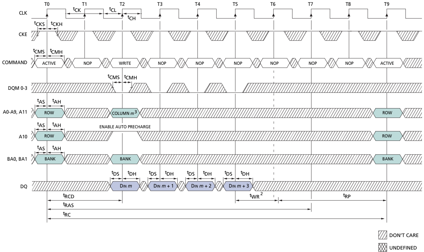
Figure 43: Write – With Auto Precharge
