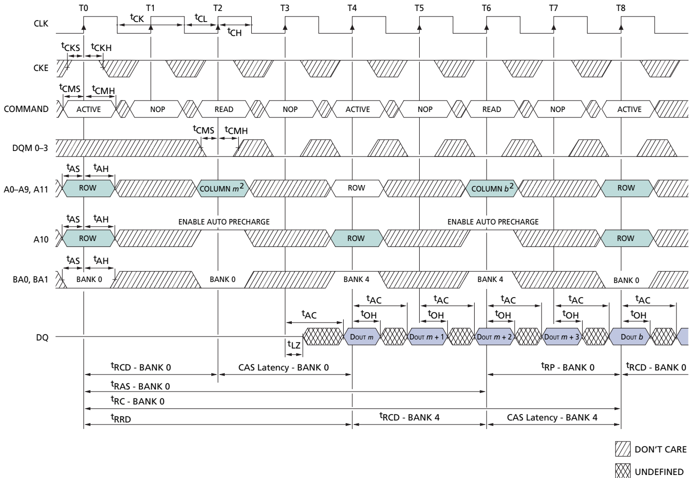
Figure 38: Alternating Bank Read Accesses
