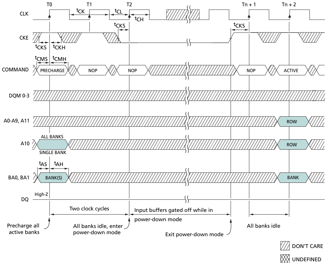
Figure 32: Power-Down Mode
