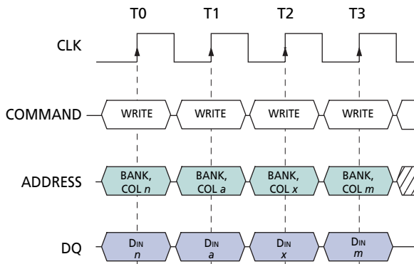
Figure 19: Random WRITE Cycles
