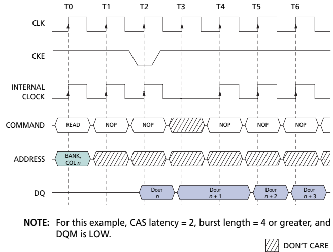
Figure 26: CLOCK SUSPEND During READ Burst
