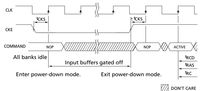
Figure 24: Power-Down
