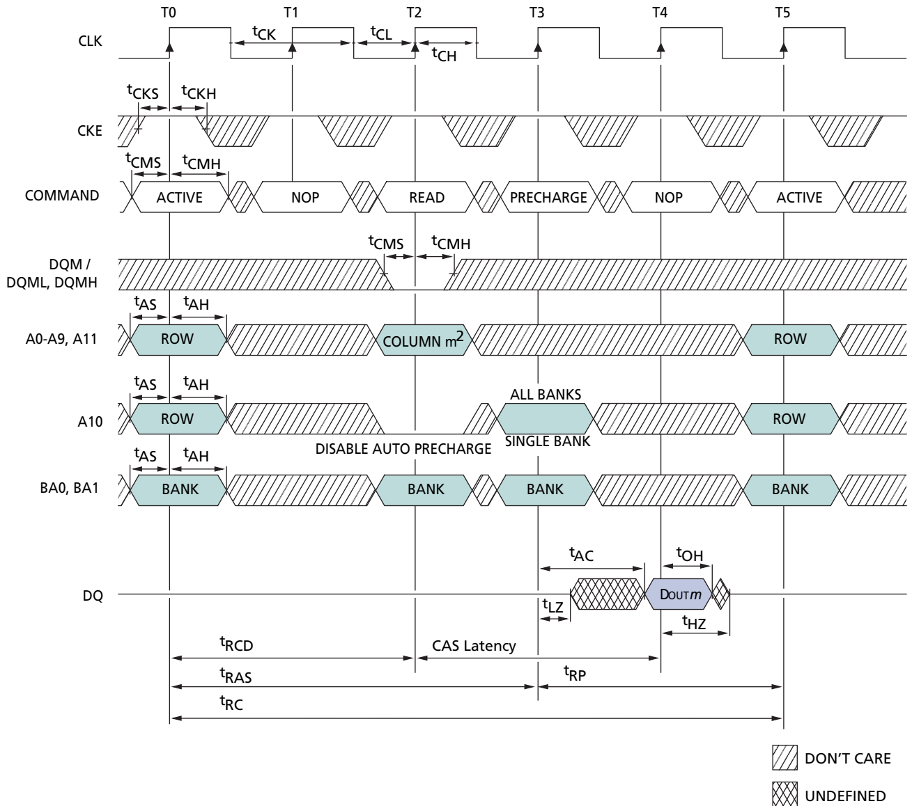
Figure 36: Single READ – Without Auto Precharge
