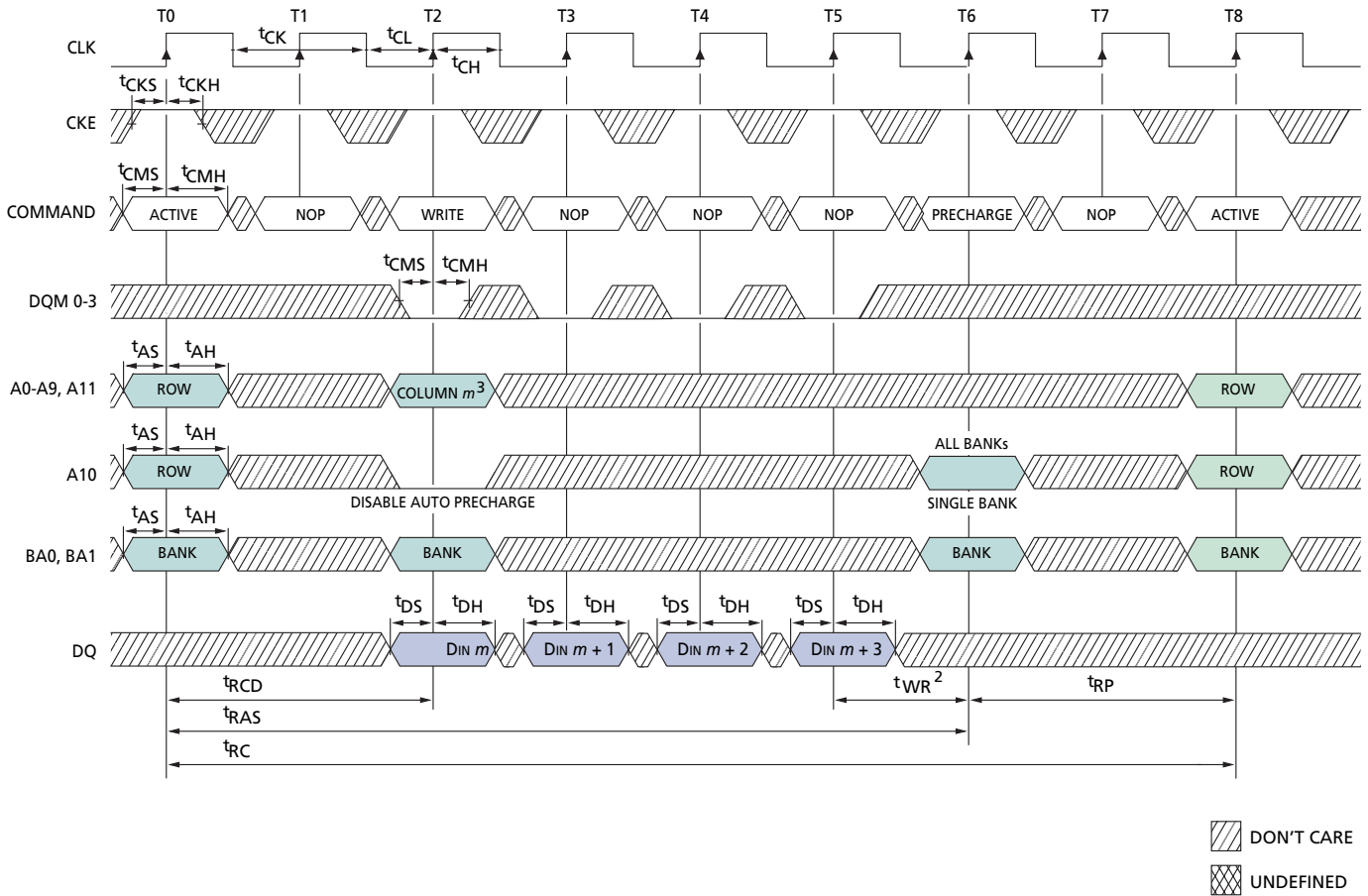
Figure 42: Write – Without Auto Precharge
