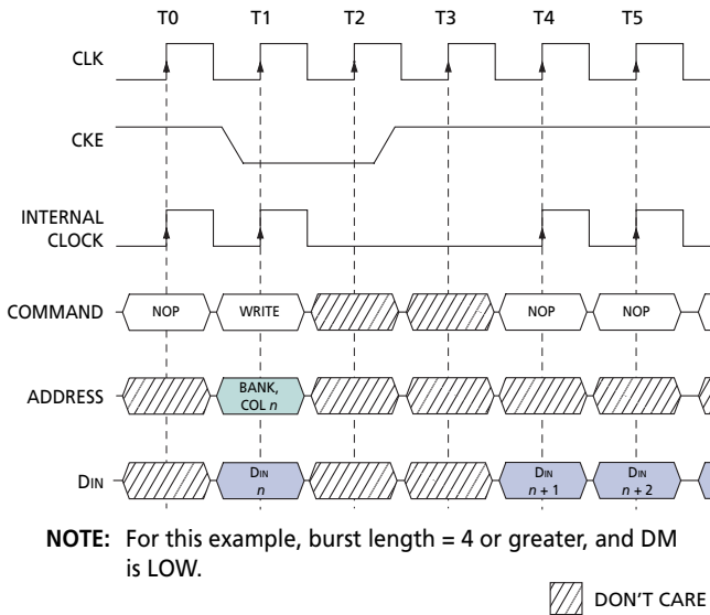
Figure 25: CLOCK SUSPEND During WRITE Burst
