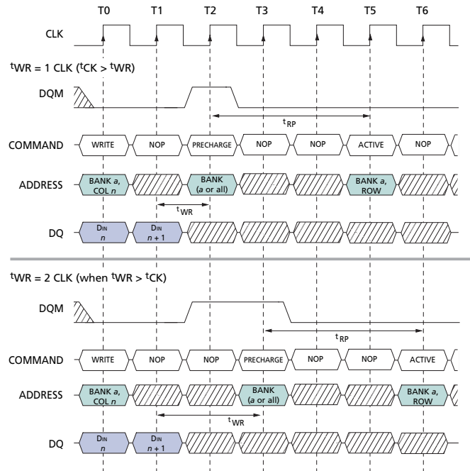
Figure 21: WRITE to PRECHARGE
