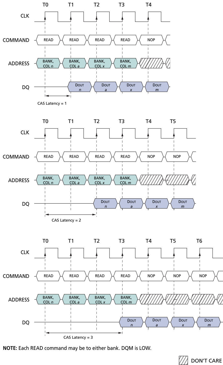
Figure 11: Random READ Accesses
