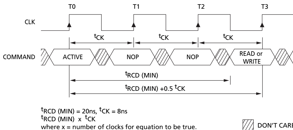
Figure 7: Example: Meeting t_{RCD}(\text{MIN}) When 2 < t_{RCD}(\text{MIN})/t_{CK} \leq 3
