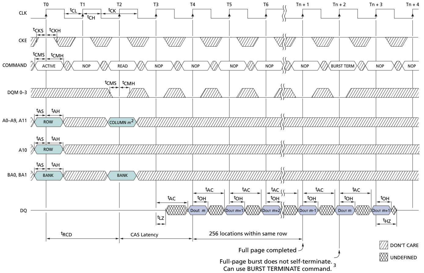
Figure 39: Read – Full-page Burst
