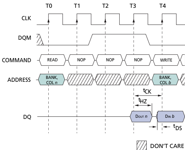
Figure 12: READ to WRITE
