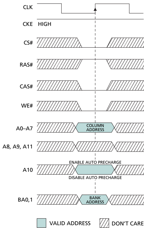
Figure 16: WRITE Command
