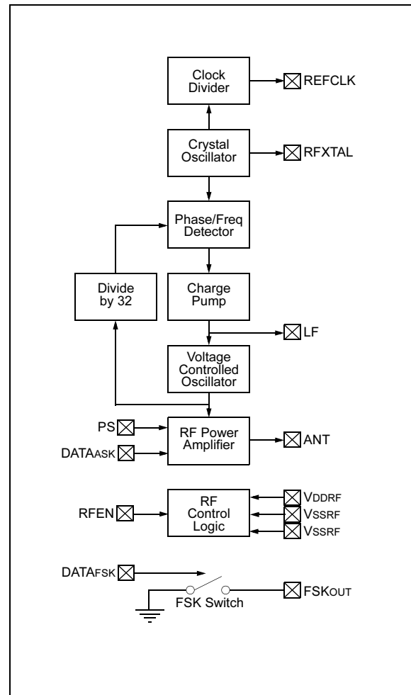
FIGURE 9-1: TRANSMITTER BLOCK DIAGRAM
