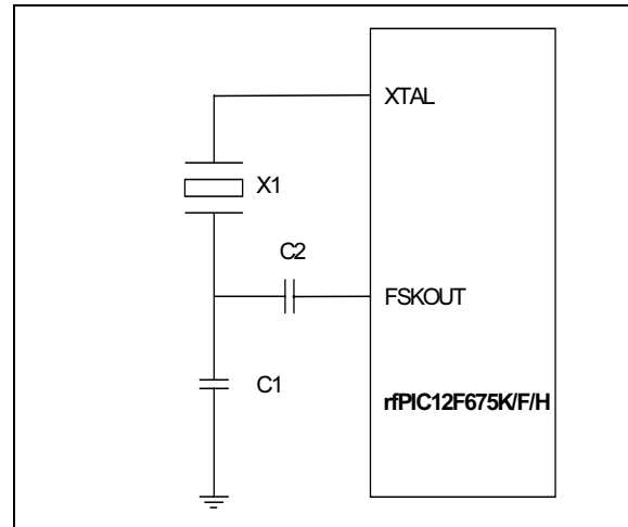
FIGURE 9-3: FSK CRYSTAL CIRCUIT
