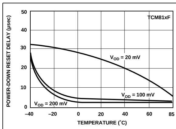
FIGURE 2-2: Power-Down Reset Delay vs. Temperature.
