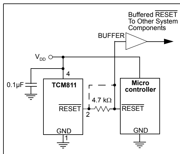
FIGURE 4-3: Interfacing the TCM811 to a Bidirectional Reset I/O.
