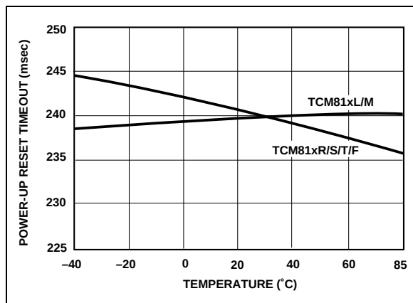
FIGURE 2-3: Power-Up Reset Timeout vs. Temperature.
