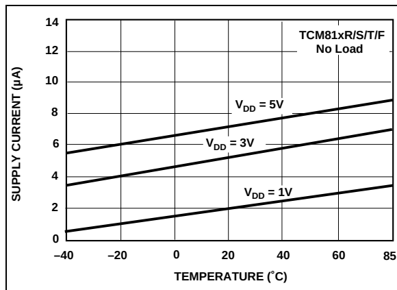
FIGURE 2-1: Supply Current vs. Temperature.
