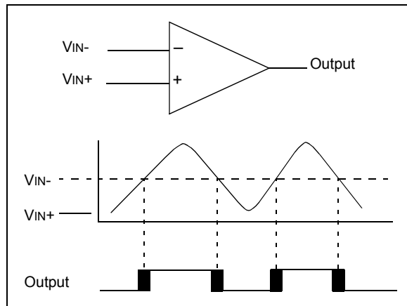
FIGURE 24-2: SINGLE COMPARATOR
