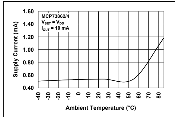
FIGURE 2-22: Supply Current ( I_{SS} ) vs. Ambient Temperature ( T_A ).
