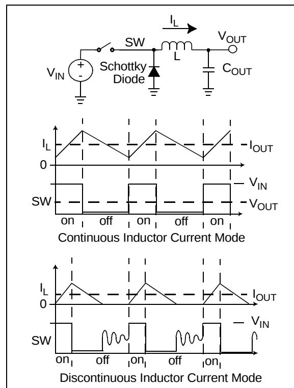
FIGURE 4-2: Step-Down Converter.
