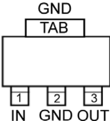
3-Pin SOT-223 (S)
