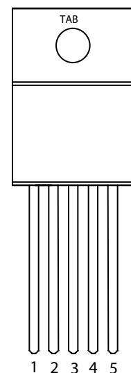
MIC29201/29202BT (TO-220-5)
