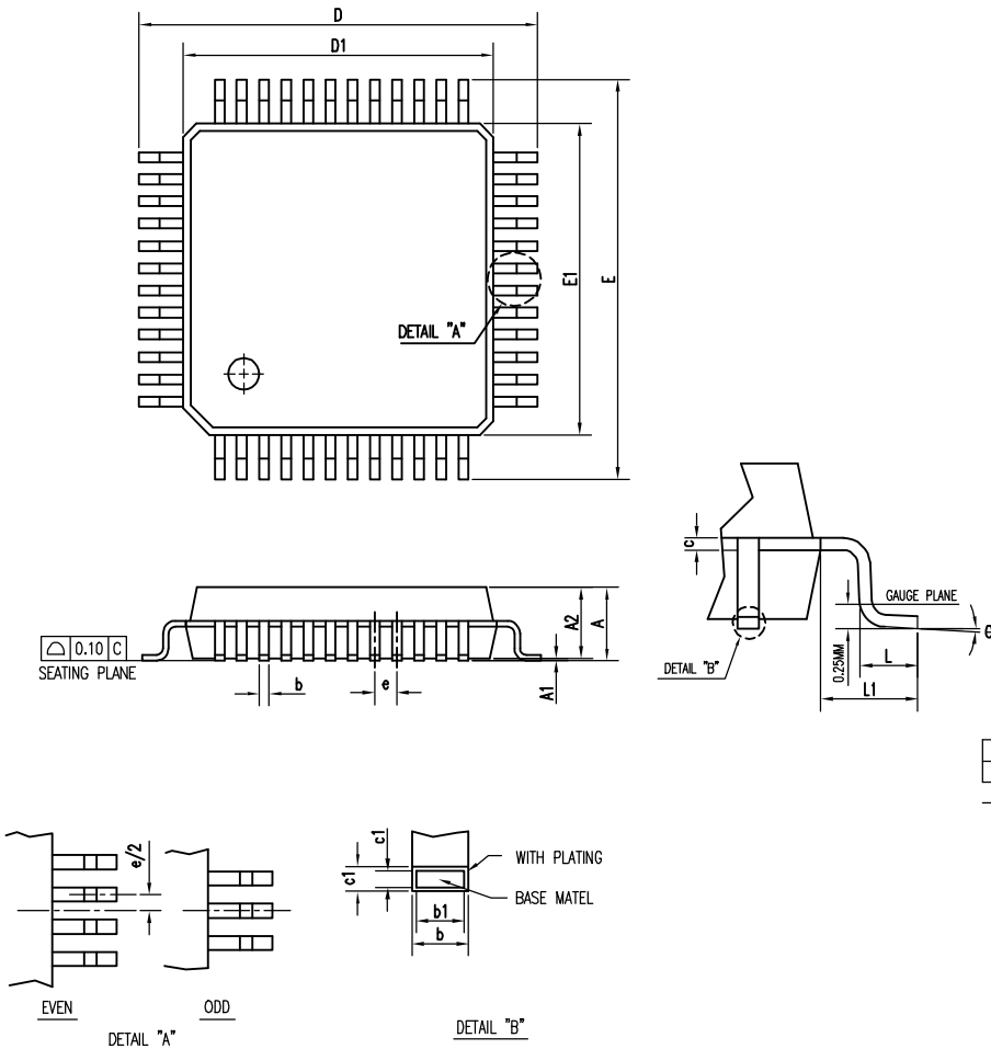
48-Pin (7mm x 7mm) LQFP
