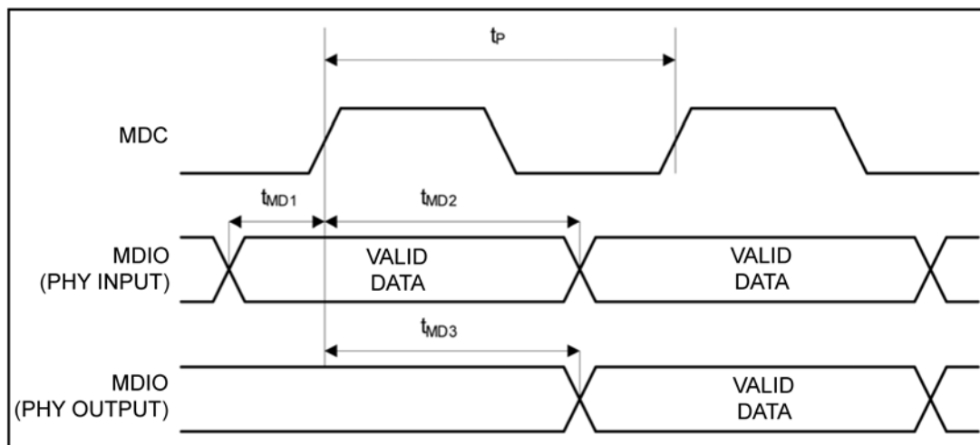
Figure 11. MDC/MDIO Timing
