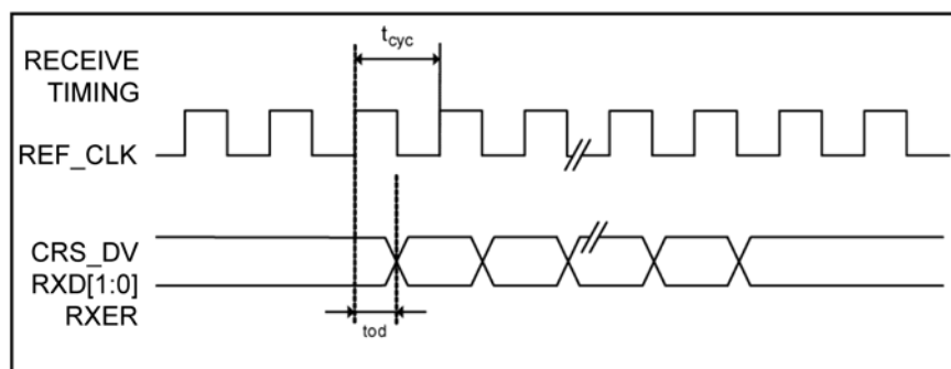
Figure 9. RMII Timing – Data Input to RMII
