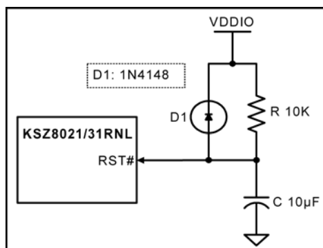
Figure 13. Recommended Reset Circuit
