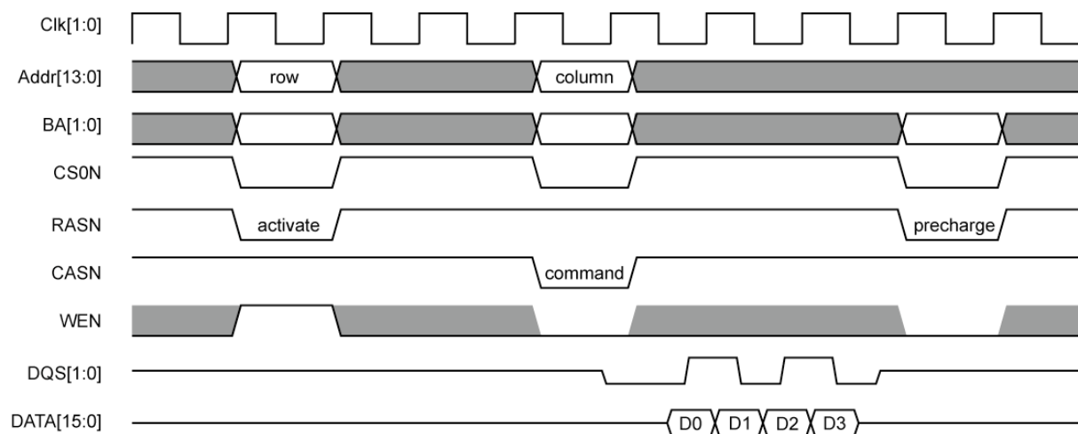
Figure 11. Burst DDR Write Timing
