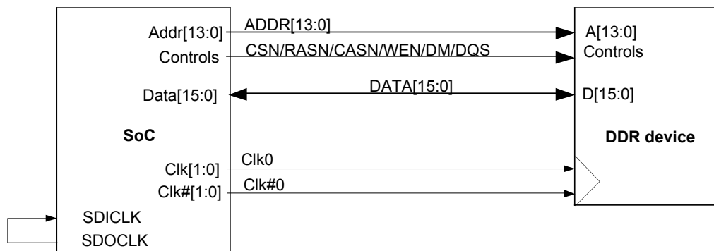
Figure 8. Single 16-bit DDR Memory Device Interface Example
