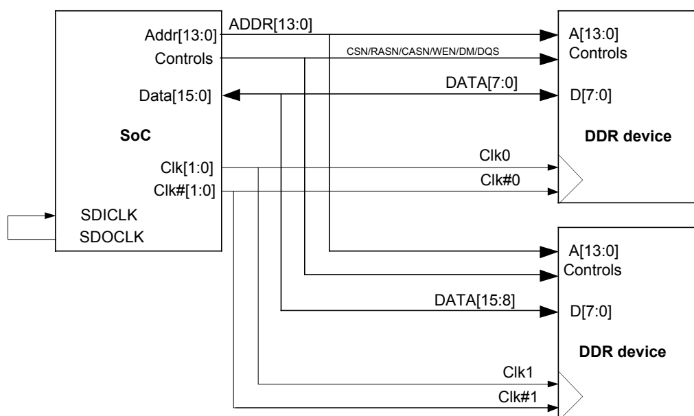
Figure 9. Two 8-bit DDR Memory Devices Interface Example
