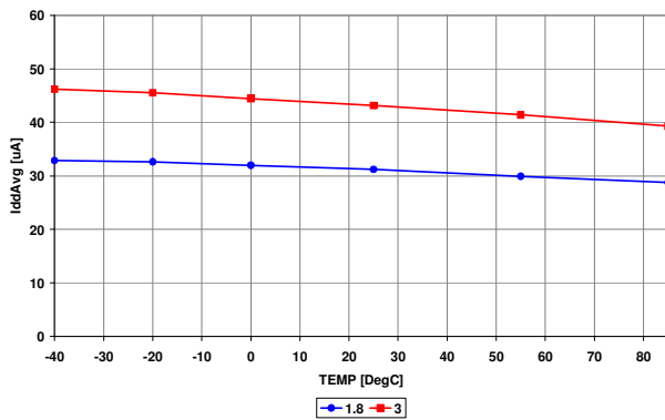
11.5 Supply Current vs. Temperature
