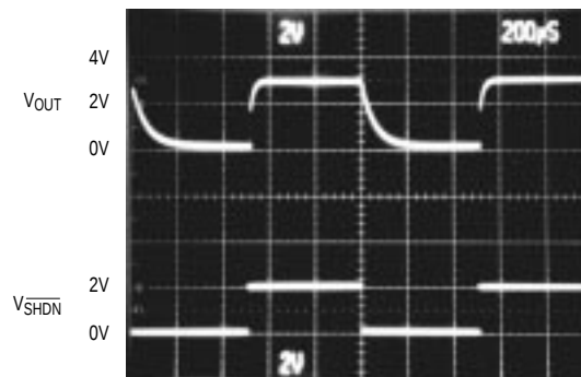
MAX8874 SHUTDOWN
