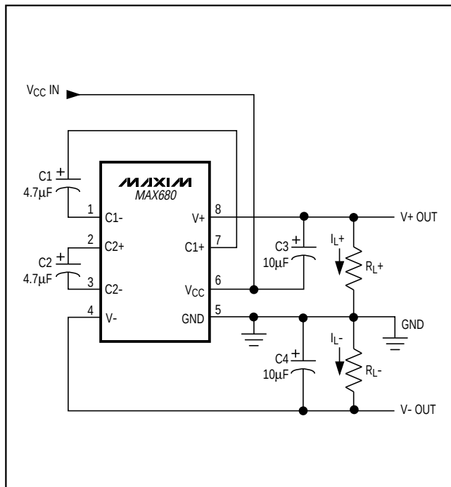
Figure 1. Test Circuit
