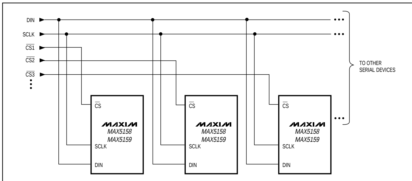
Figure 8. Multiple MAX5158/MAX5159s Sharing a Common DIN Line
