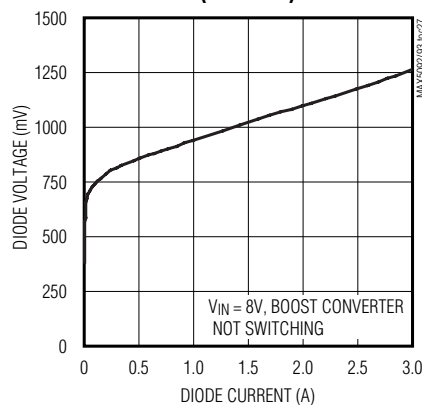
INTERNAL BOOST DIODE FORWARD DROP (MAX5092)
