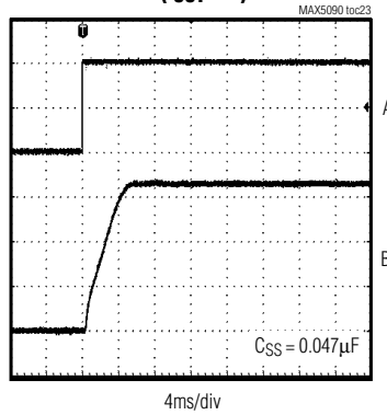
STARTUP WAVEFORM ( I_{OUT} = 0 )
