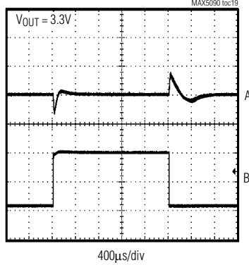
LOAD-TRANSIENT RESPONSE (MAX5090AATE)
