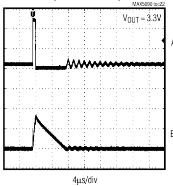
LX WAVEFORM (MAX5090AATE)
