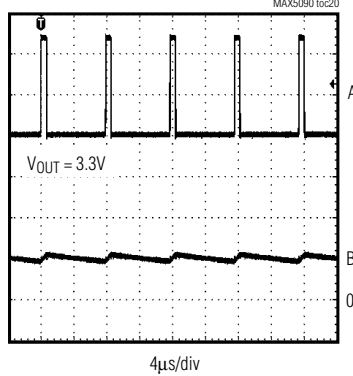
LX WAVEFORMS (MAX5090AATE)
