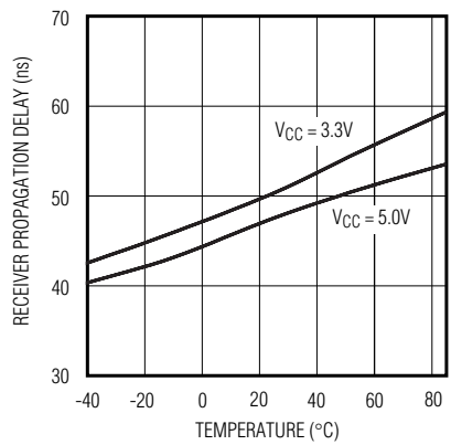
RECEIVER PROPAGATION DELAY vs. TEMPERATURE
