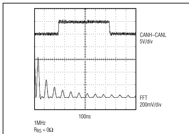
Figure 7. Output Bus High-Speed Mode at 2Mbps
