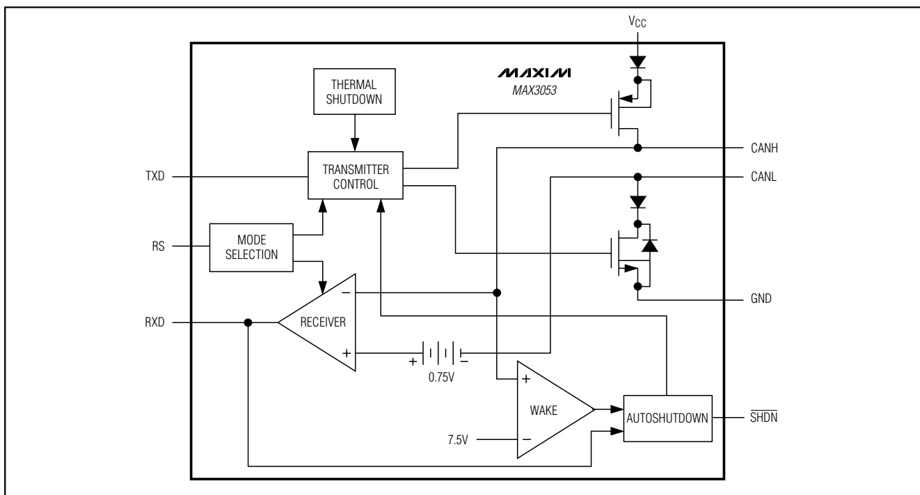
Figure 4. Block Diagram
