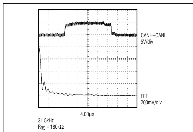
Figure 5. Output Bus in Slope Control Mode at 62.5kbps
