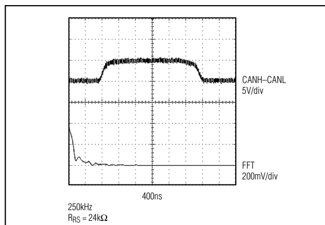
Figure 6. Output Bus in Slope Control Mode at 500kbps
