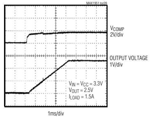
SOFT-START WAVEFORMS
