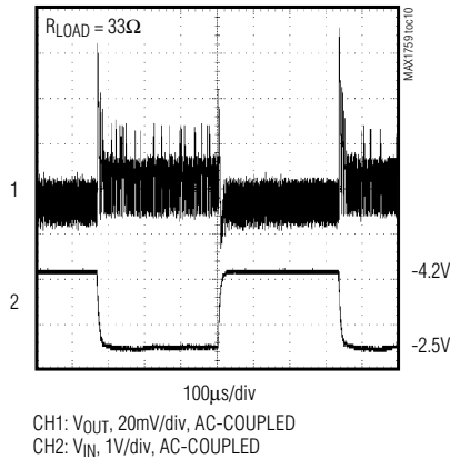
LINE-TRANSIENT RESPONSE
