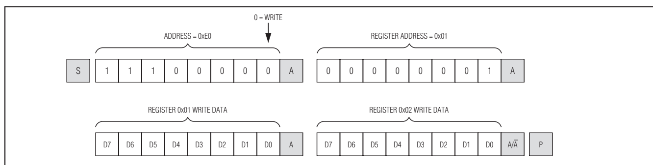
Figure 18. Format for Writing to Multiple Registers. In this example, registers 0x01 and 0x02 are written in sequence.
